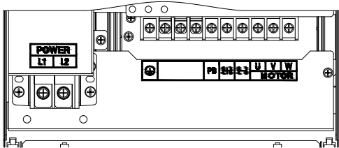
4.0-11kW Main circuit terminal
