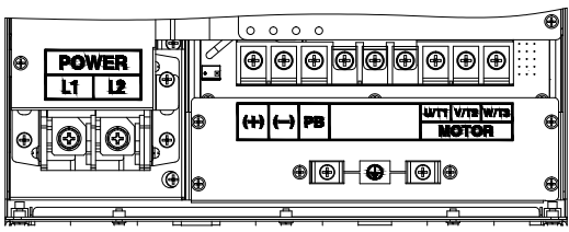
15-22kW Main circuit terminal
