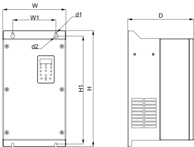
Dimension Drawing
