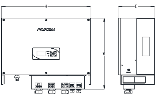
Schematic diagram of product size (≥30kW)
