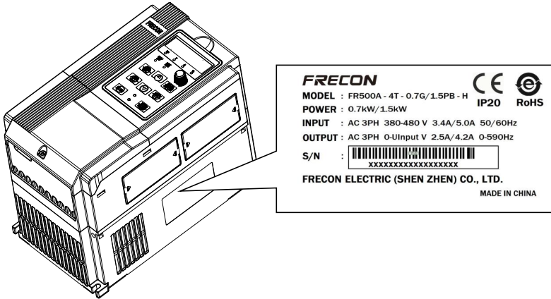
Fig.1-1 Nameplate information
