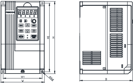
Fig 1-5 0.7~22kW Wall installation diagram
