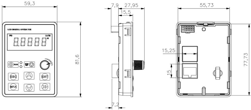
Fig 1-11- 0.7~5.5KW Keyboard size diagram
