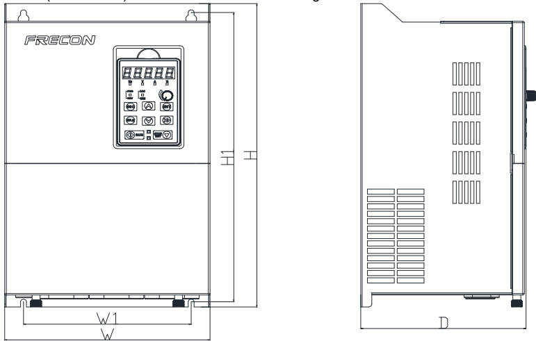
Fig 1-6 30~280KW Wall installation diagram
