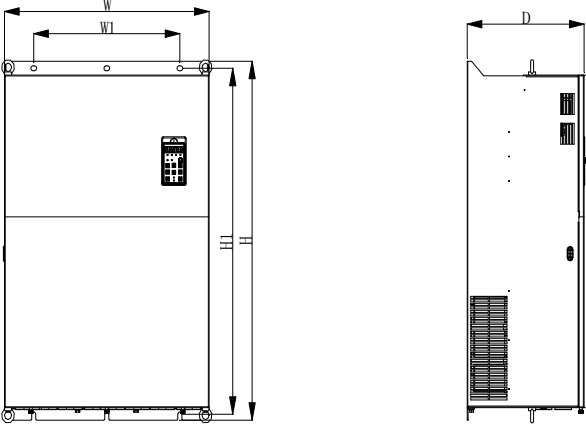
Fig 1-7 315~400KW Wall installation diagram
