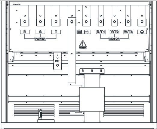
◆FR500A-4T(800～1120KW) Main Circuit Terminals:
