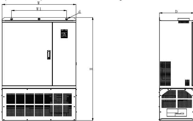
Fig 1-8 450~560KW Wall installation diagram
