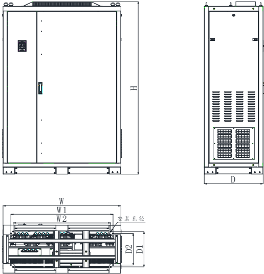
Fig 1-10 800~1120KW Wall installation diagram
