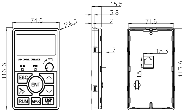
Fig 1-12- 7.5~450KW Keyboard size diagram
