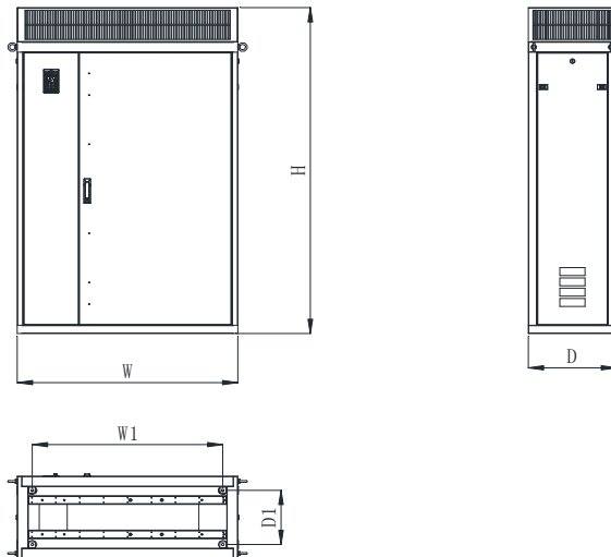
Fig 1-9 630~710KW Wall installation diagram
