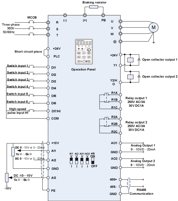
Fig.2-1 FR500A&FR510A Inverter wiring diagram
