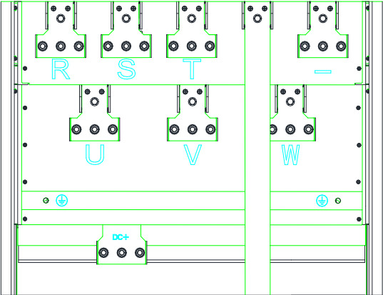
◆FR500A-4T(800～1120KW) Main Circuit Terminals:
