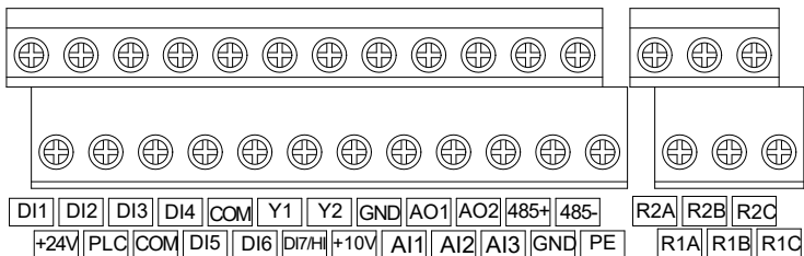
Fig.2-2b Control circuit terminals
